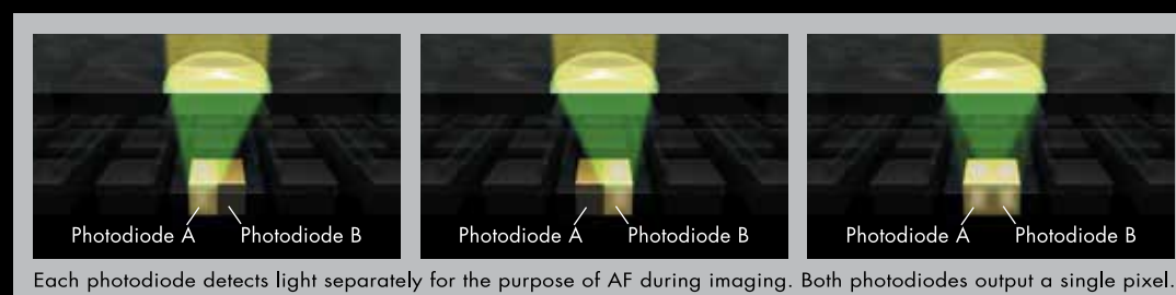
Each photodiode detects light separately for the purpose of AF during imaging. Both photodiodes output a single pixel.
